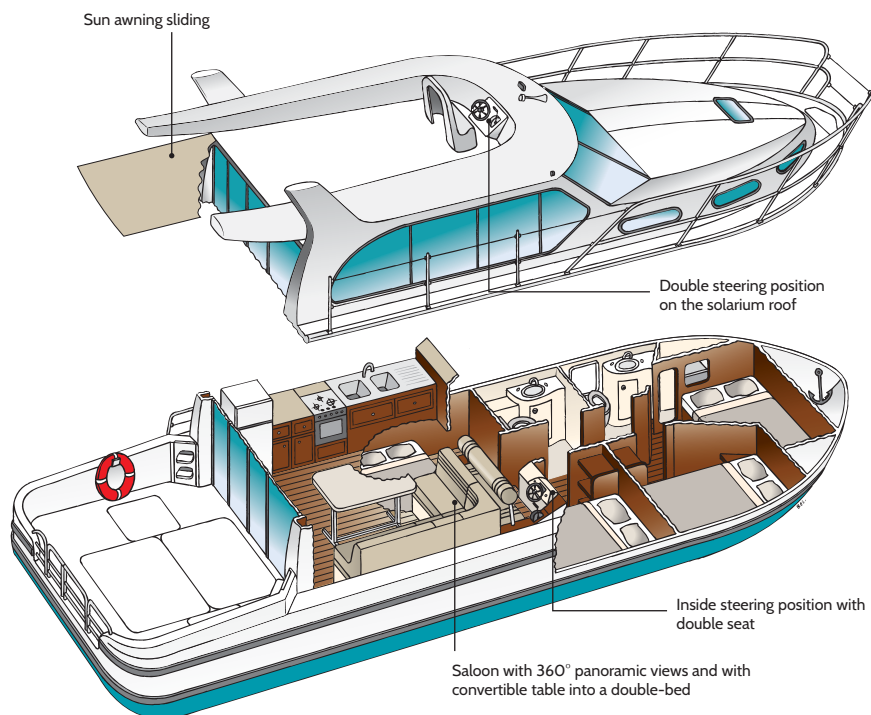
3D Model of boat: Nicols® 1170
